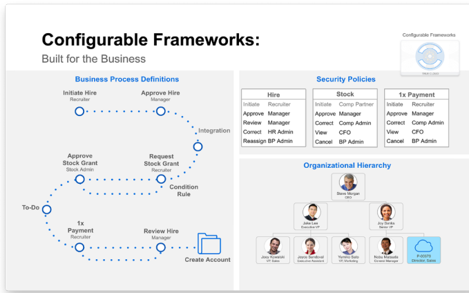
Configurable frameworks.
